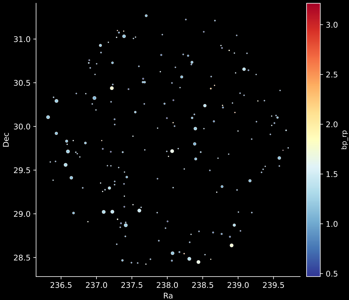
APOGEE DR17 Field: [196+42_MGA] Stars: 196
