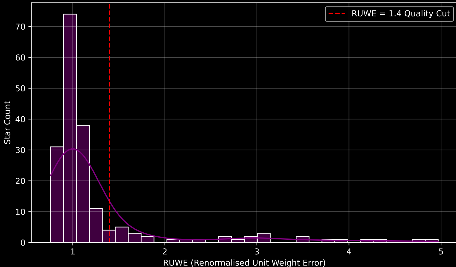
GAPOGEE DR17 Field [196+42_MGA] RUWE Distribution (n= 187)
