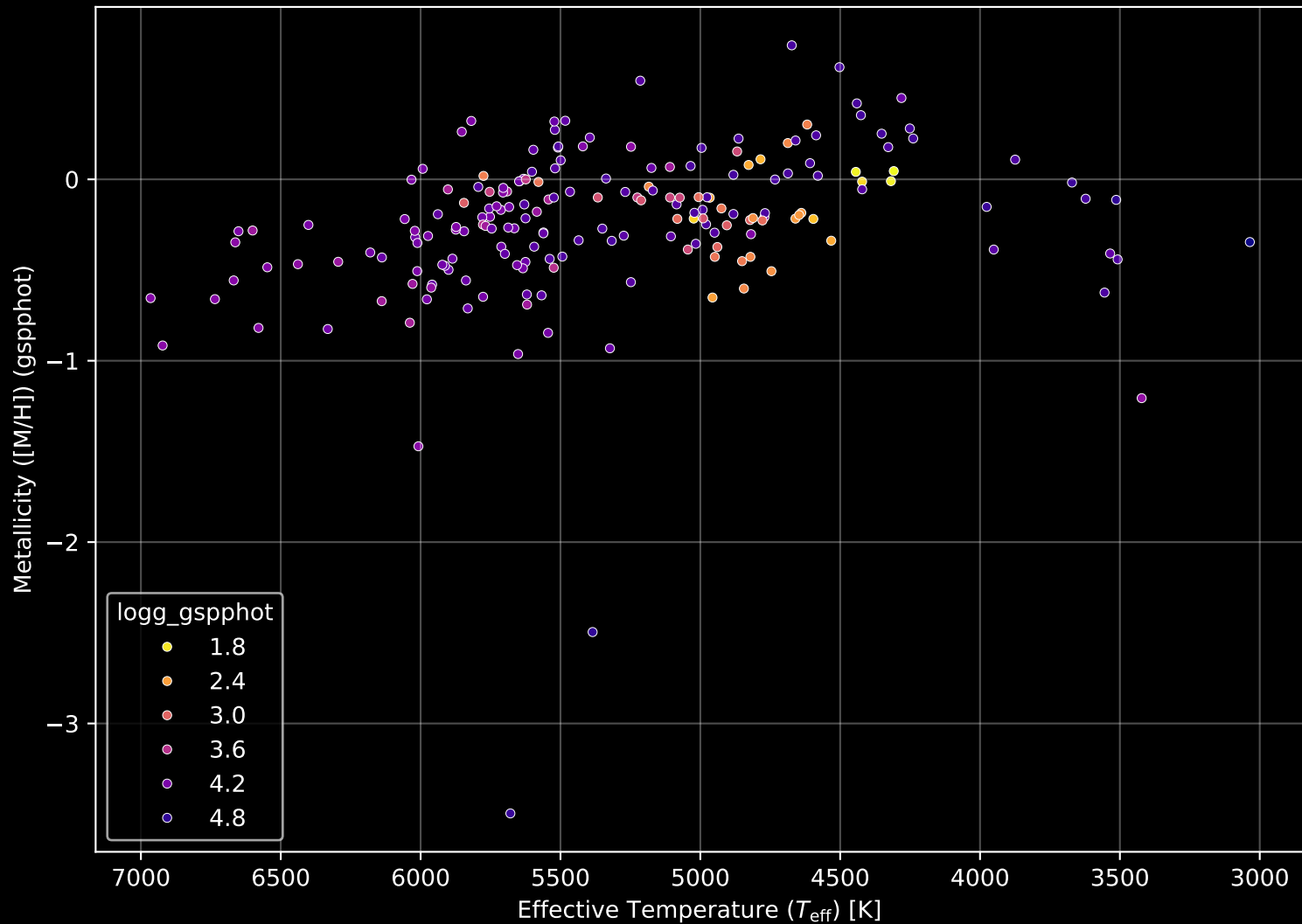
APOGEE DR17 Field: [196+42_MGA] Stellar Population Parameters (n= 196)
