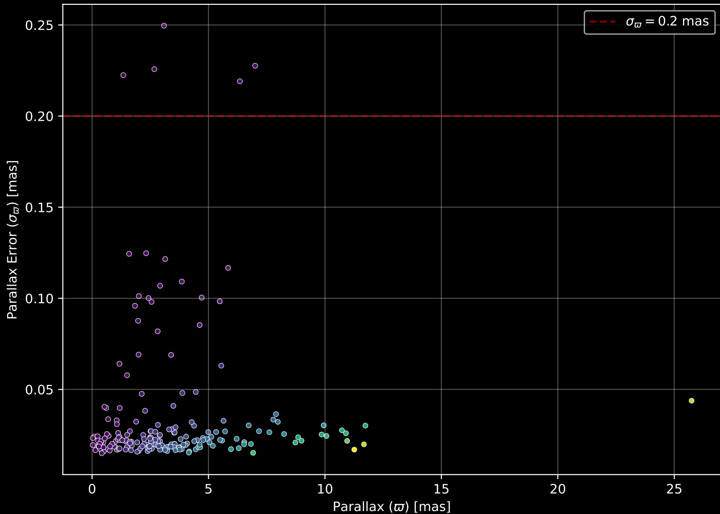
APOGEE DR17 Field: [196+42_MGA] Parallax Quality (n= 196)
