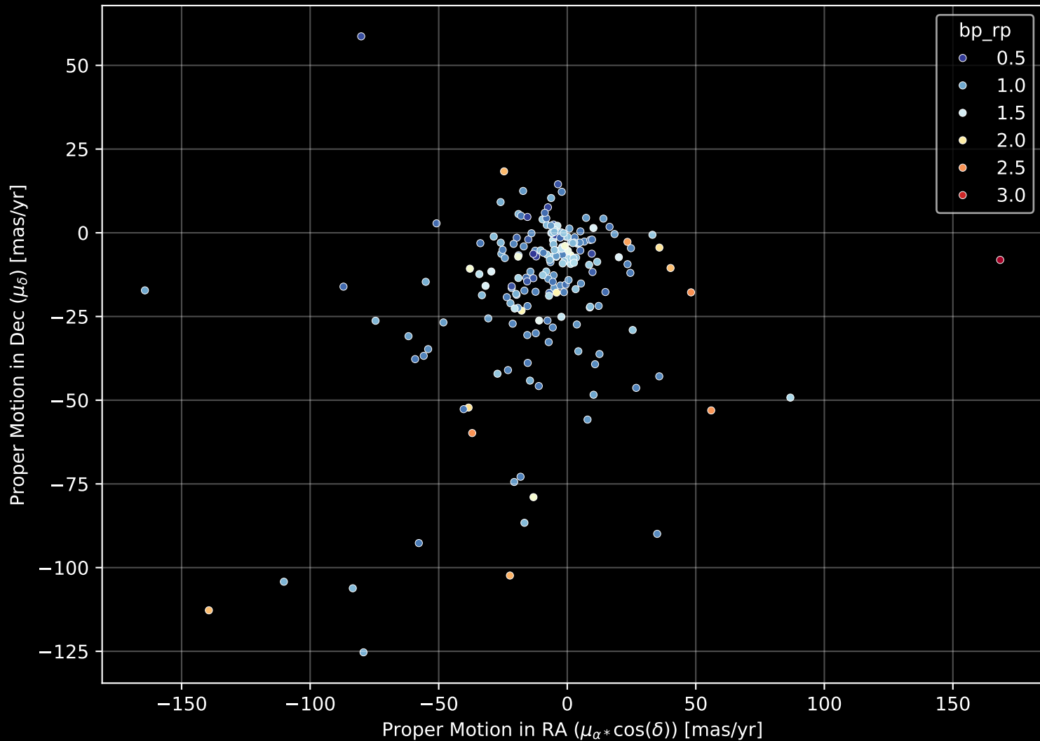
APOGEE DR17 Field: [196+42_MGA] Proper Motion Diagram (n= 196)
