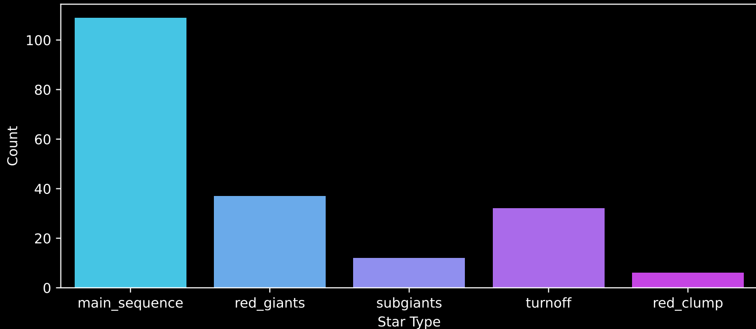
APOGEE DR17 Field: [196+42_MGA] Count plot of Star Type
