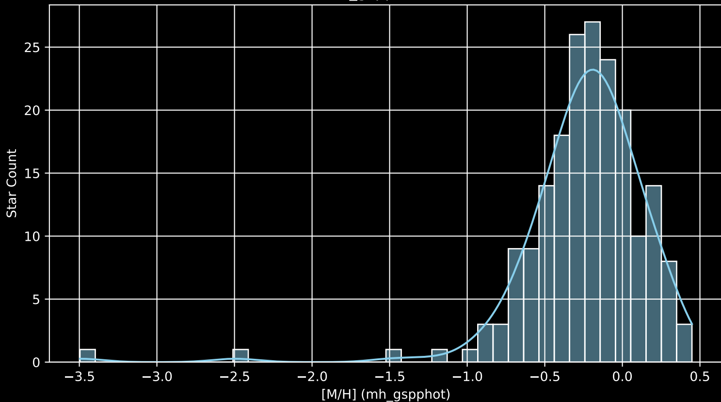
APOGEE DR17 Field: [196+42_MGA [M/H] (mh_gspphot) (n= 193)
